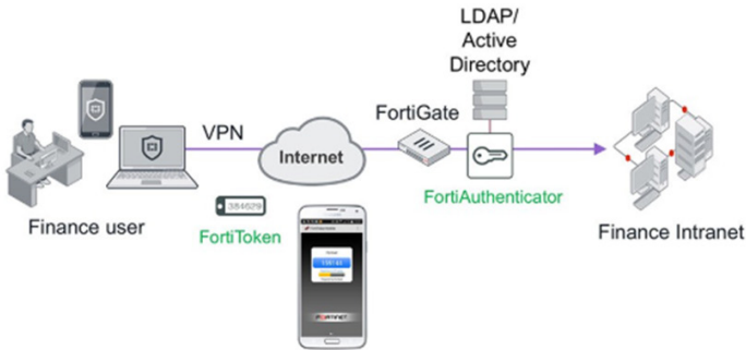
Figure 1: A typical Fortinet ZTA user identity and access management implementation.
